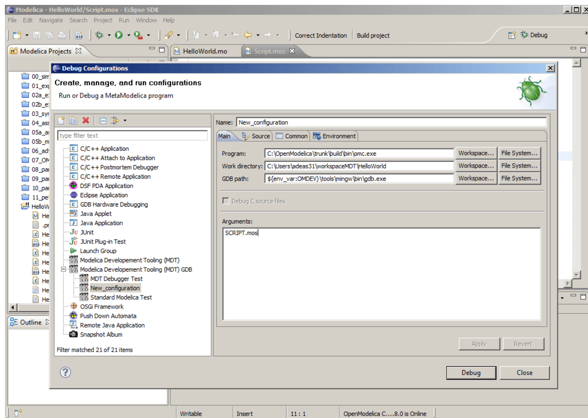
Figure 19.3: Creating the Debug Configuration.
